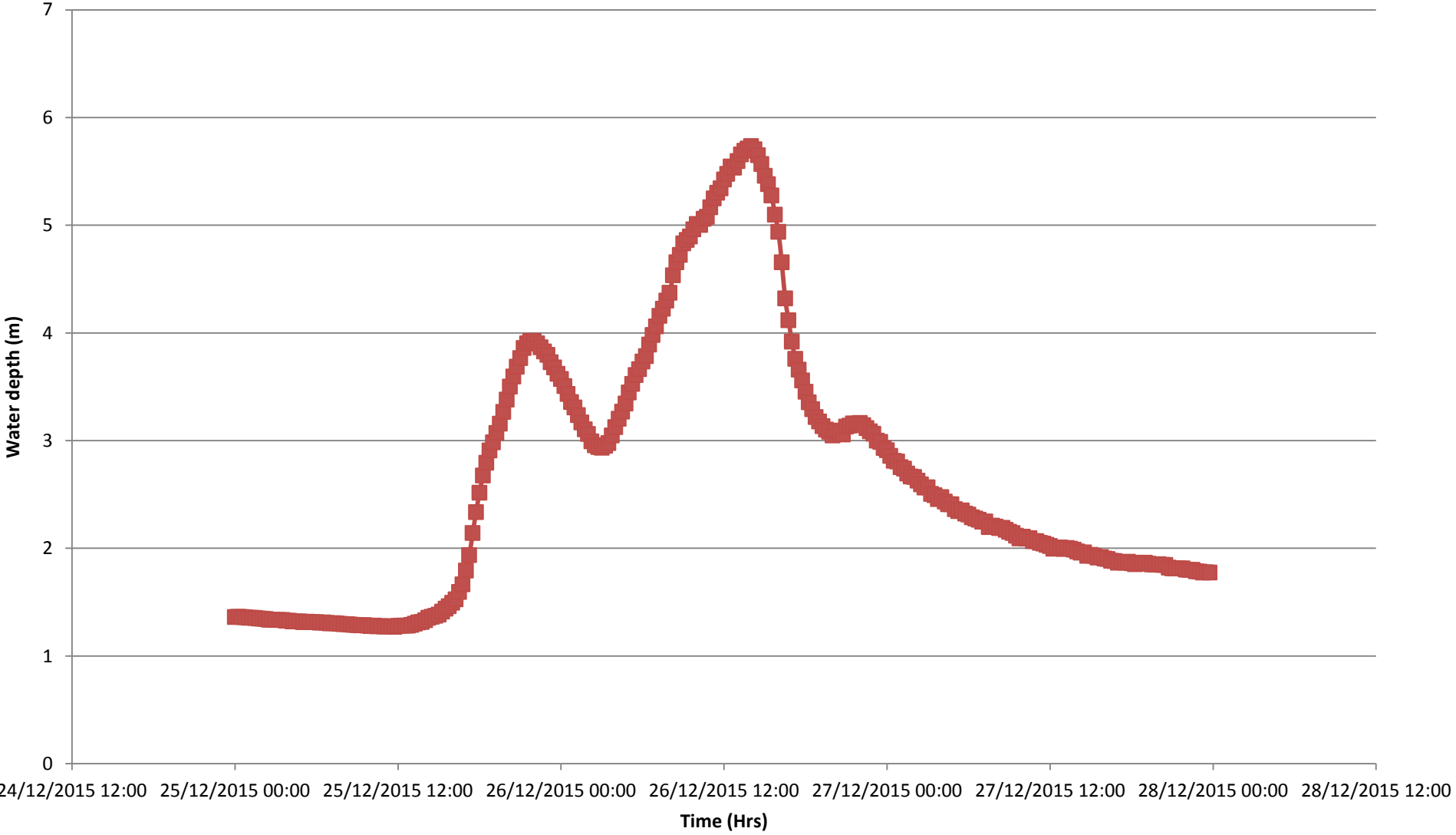
Graph 1: Caldene Avenue - Mytholmroyd Water depth (m) v Time (Hrs)
