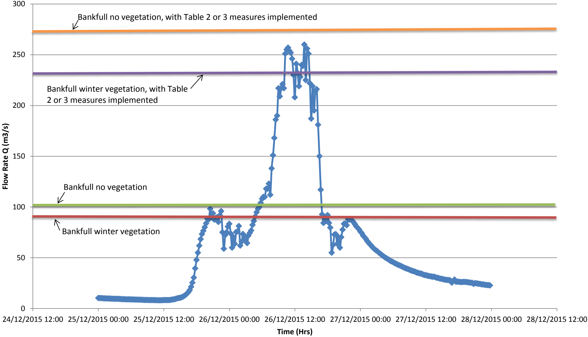
Graph 2: Caldene Avenue - Mytholmroyd Flow rate (Q) v Time (Hrs)
